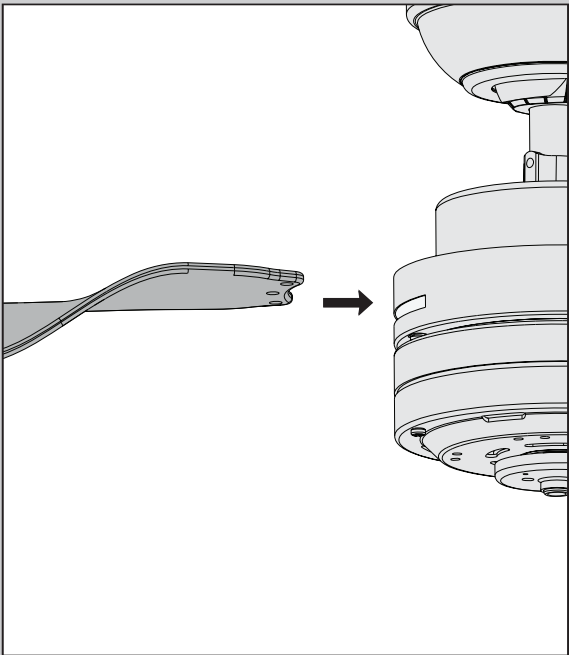
Insert each blade into a slot. Align the holes on the blade with the holes on the blade ring.
