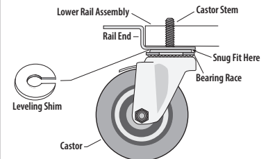
Fig. 7. Install shim(s).
