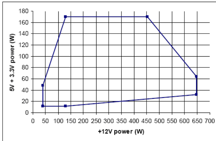
Figure 7 750W Cross loading graph
