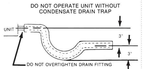
FIGURE 11 CONDENSATE DRAIN
