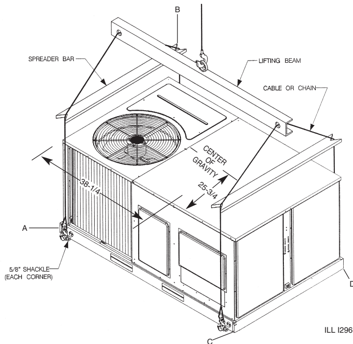
FIGURE 7 PACKAGE AIR CONDITIONER – RIGGING FOR LIFTING
