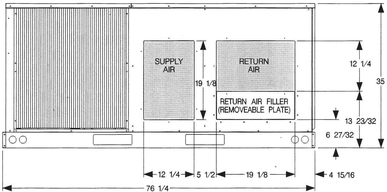
FIGURE 4 UNIT DIMENSIONS
