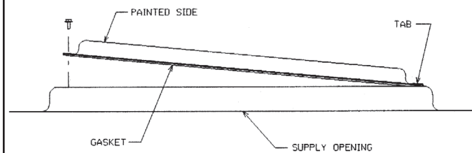
FIGURE 10 COVER GASKET DETAIL
