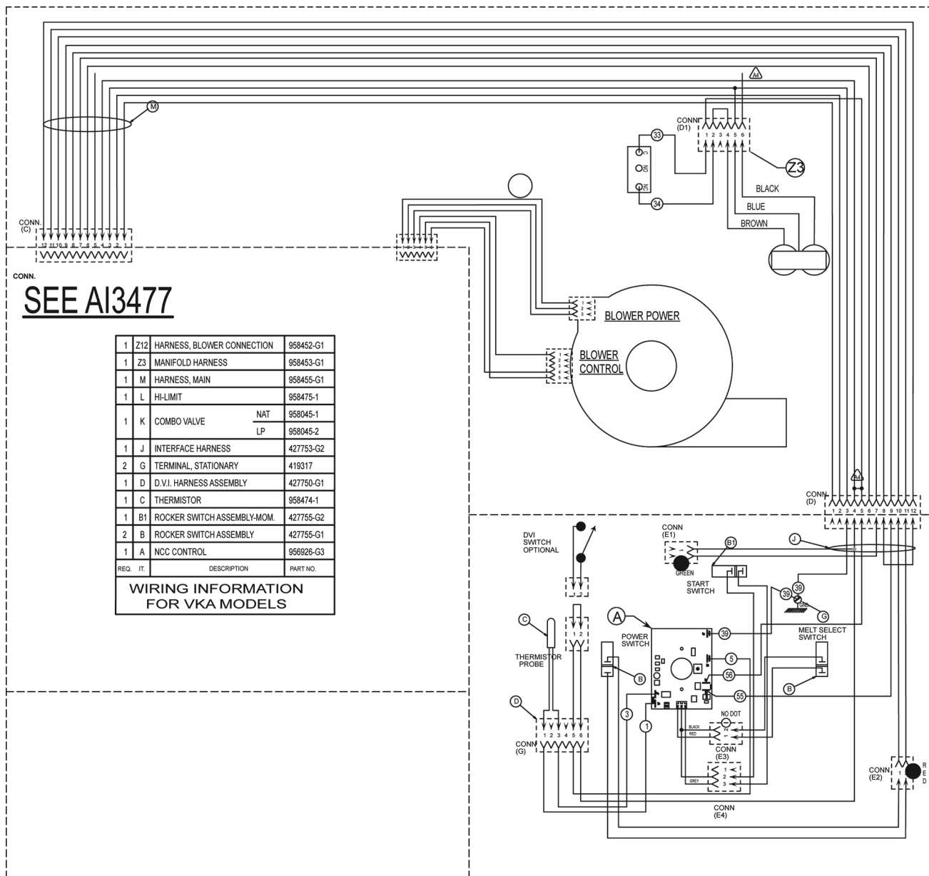
WIRING DIAGRAM ANALOG CONTROL - NO OPTIONS
