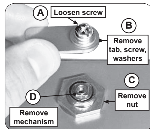
Fig. 4-5 Locking / unlocking
