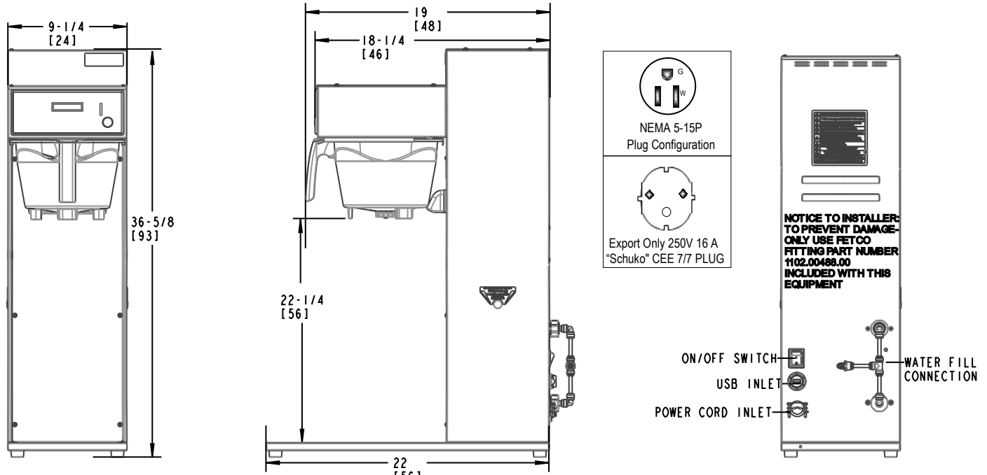
TBS-1221/1222 Front
