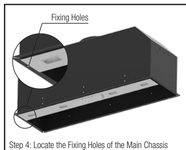
Step 4: Locate the Fixing Holes of the Main Chassis
