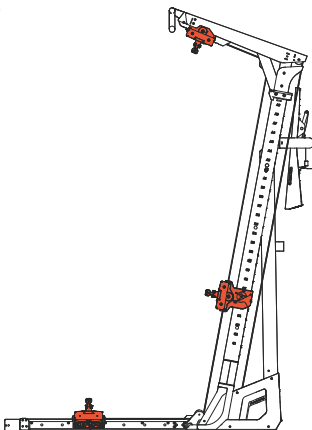
○ Schematic Diagram of Third-Party Connector Usage
