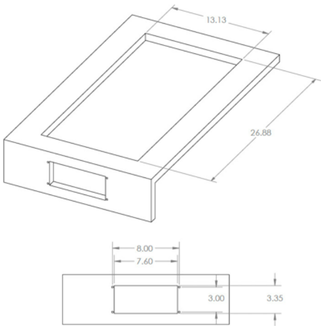
Top Mount
