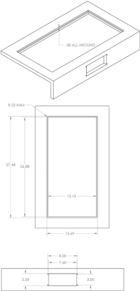
Flush Mount
