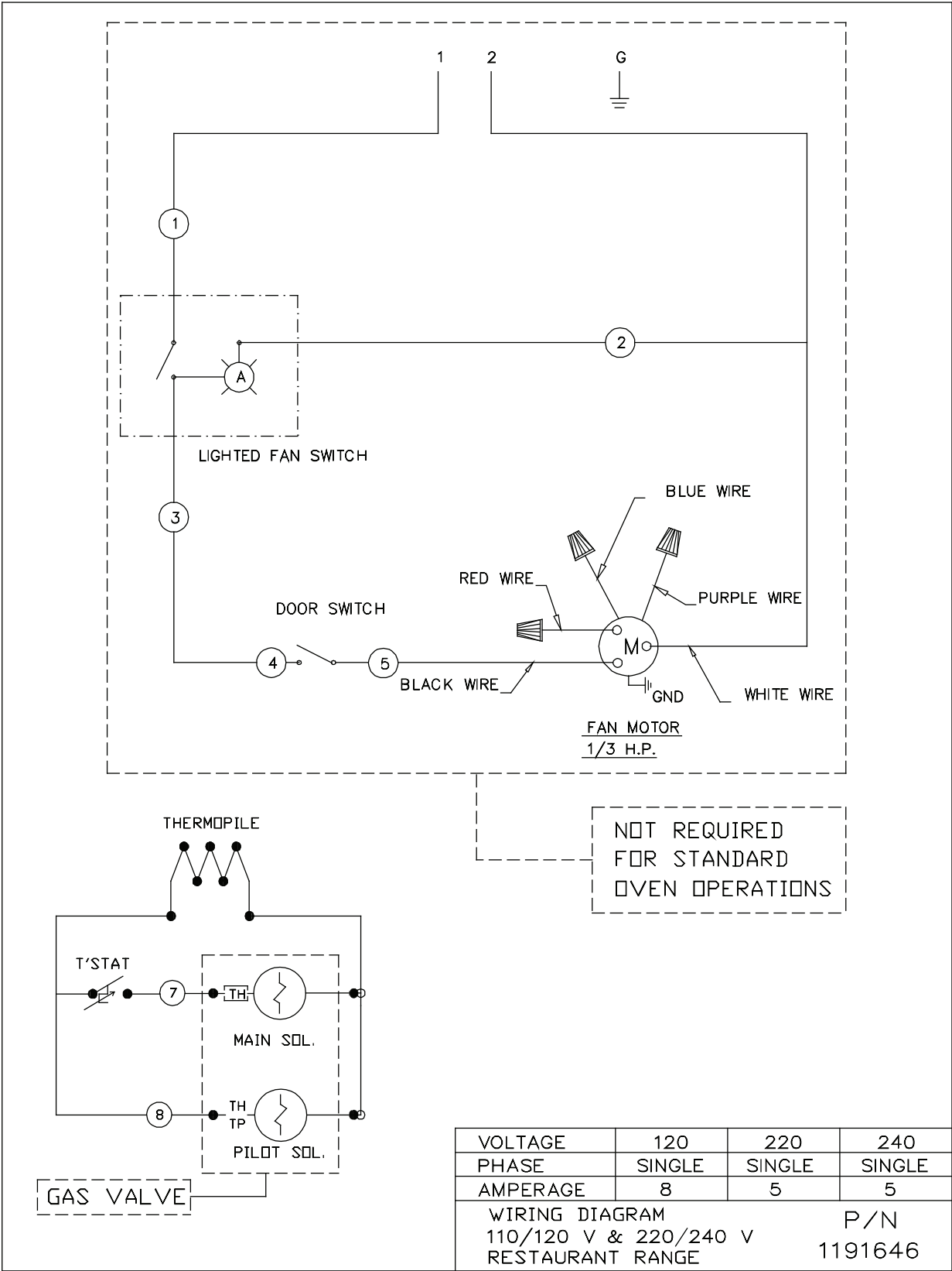
Figure 12 Wiring Diagram for Gas Oven
