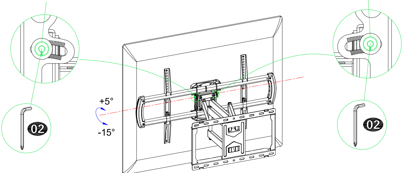
Tilting bolts
