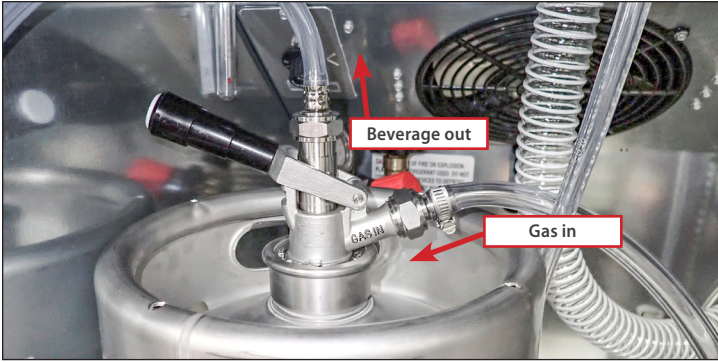
Fig. 11. Installed and connected tapper.
