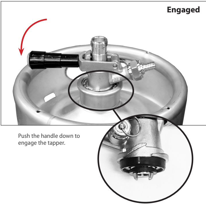
Fig. 12. Engaged tapper vs. disengaged tapper
