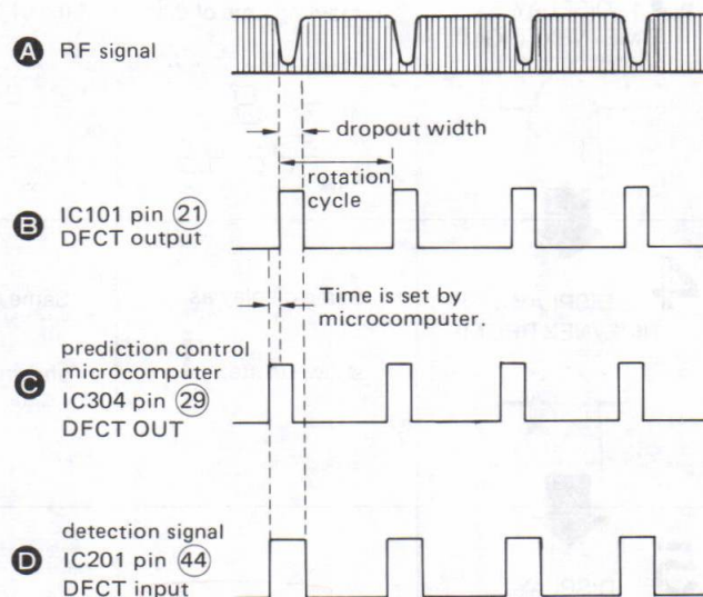
Fig. 2 Defect Detection Waveforms
