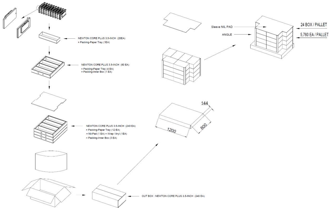
Figure 22. 3.5" PACKING-DIAGRAM (1,200 X 800)
