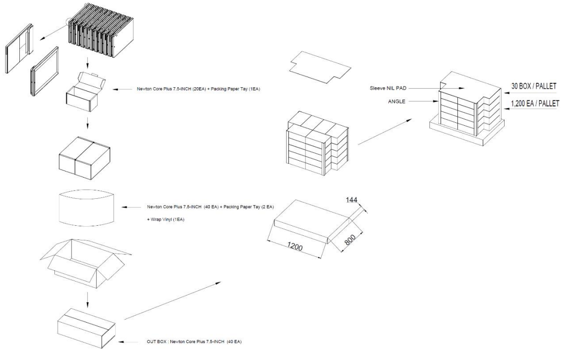
Figure 28. 7.5" PACKING-DIAGRAM (1,200 X 800)
