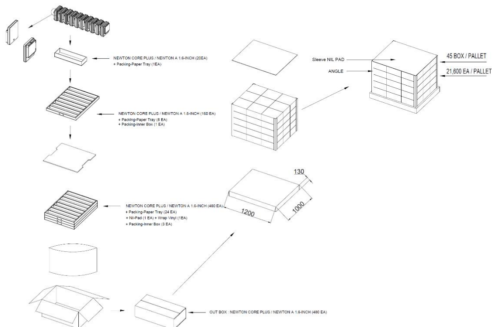
Figure 15. 1.6" PACKING-DIAGRAM (1,200 X 1,000)
