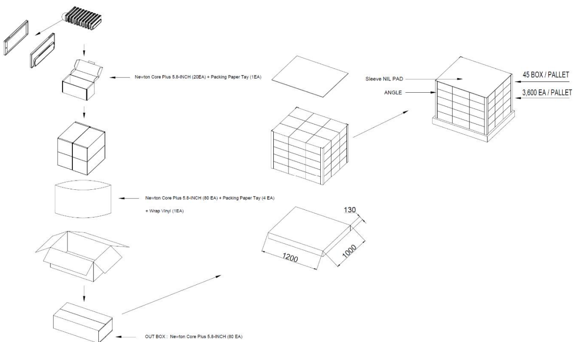
Figure 27. 5.8" PACKING-DIAGRAM (1,200 X 1,000)
