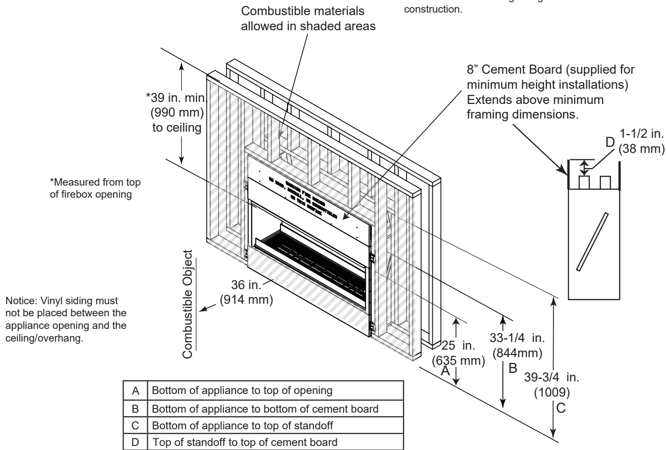
Figure 3.3. Appliance Locations and Framing Dimensions - ODLANAIGST-48
