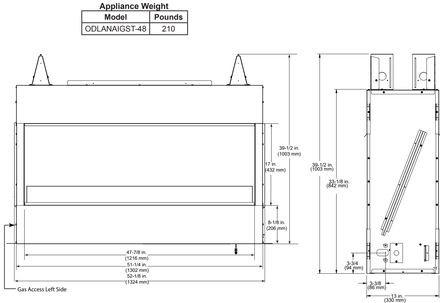
Figure 3.1. Appliance Dimensions – ODLANAIGST-48
