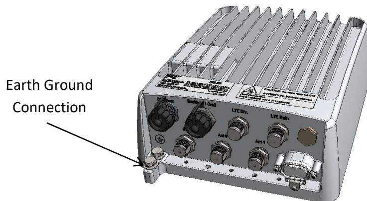
Figure 7: Chassis Ground Connection
