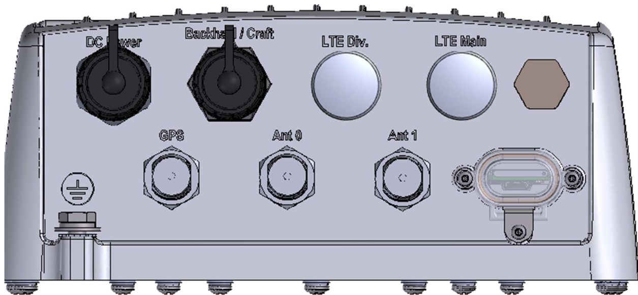
Figure 4: KONA Mega Gen3 Gateway, 2x LoRa, Ethernet backhaul only
