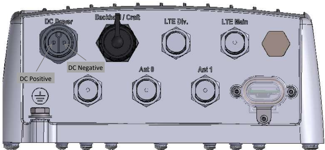
Figure 8: Direct DC Power Connection Polarity
