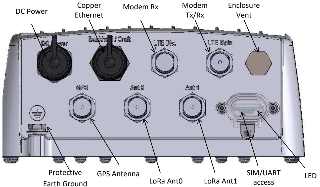
Figure 2: KONA Mega Gen3 Gateway, 2x LoRa, LTE backhaul
