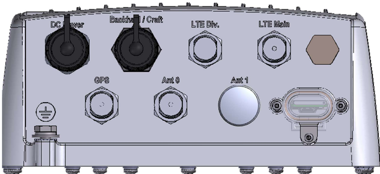
Figure 3: KONA Mega Gen3 Gateway, 1x LoRa, LTE backhaul
