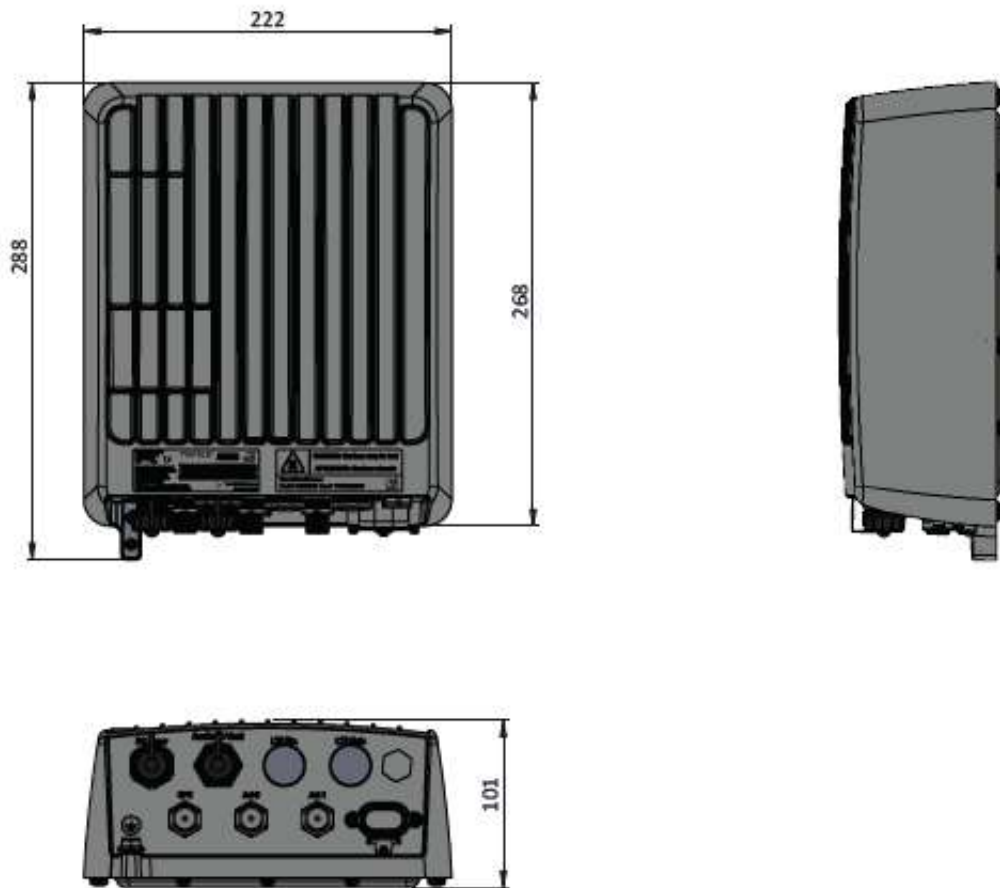
Figure 1: KONA Mega Gen3 Gateway Common Dimensions
