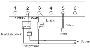
ELECTRONIC THERMOSTAT SF-102SBQ
