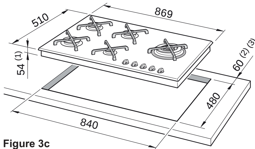
Model: DEGH90BG
