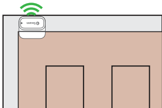
Door installation
