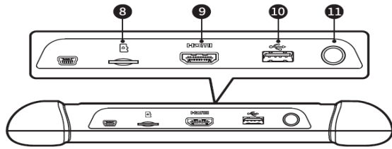
Figure 2-3 Tablet Top View
