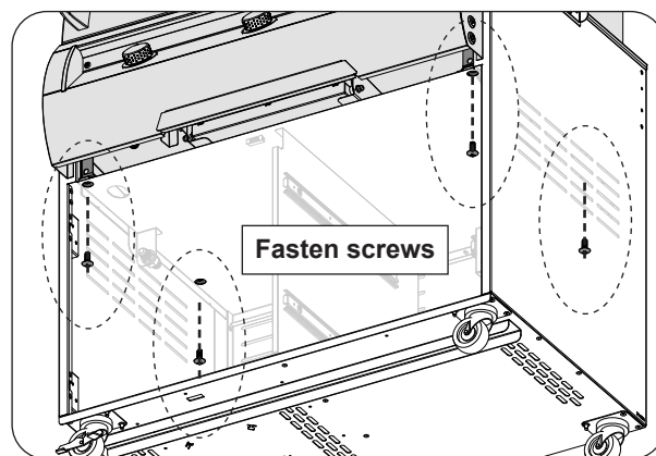
Fig. 11-4 Secure appliance to cart base
