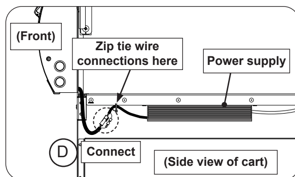
Fig. 11-3 Zip tie electrical connections
