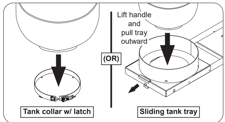
Fig. 5-2 Place cylinder
