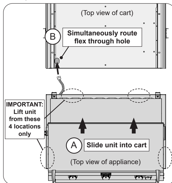
Fig. 11-1 Begin appliance installation
