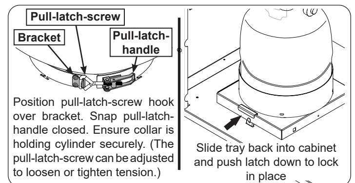
Fig. 5-4 Lock cylinder in place
