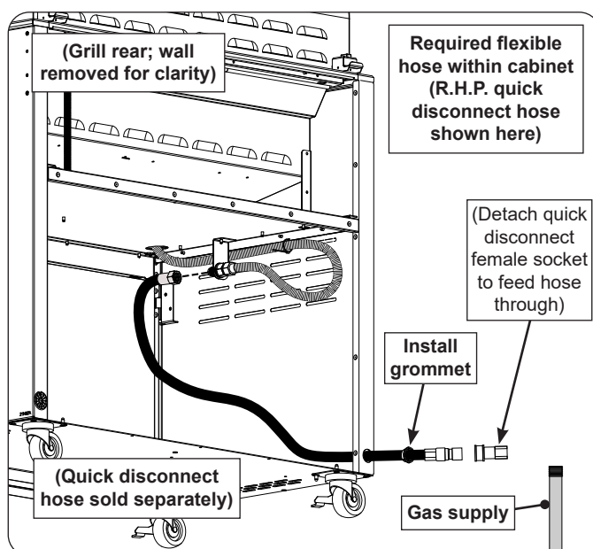
Fig. 12-2 Flexible hose assembly detail
