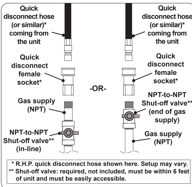
Fig. 12-3 Connecting to a gas line
