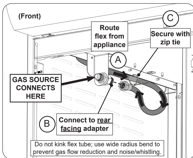
Fig. 12-1 Connect appliance flex to adapter
