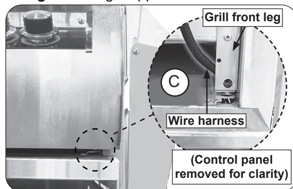
Fig. 11-2 Route wire harness
