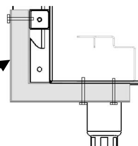
Cutaway side view
