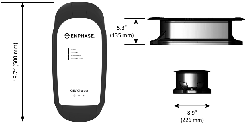
Figure 13: Enclosure Dimensions
