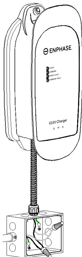
Figure 6: Wiring the EVSE in a Junction Box
