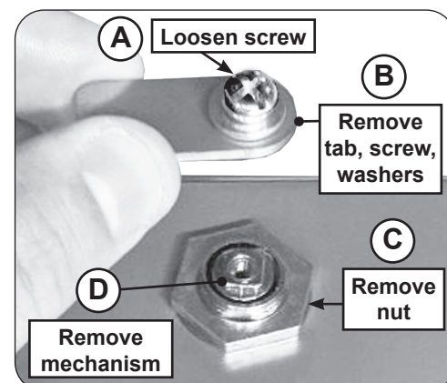
Fig. 4-5 Locking / unlocking
