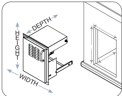
Fig. 4-6 Cut-out diagram
