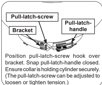
Fig. 4-7 Secure L.P. cylinder
