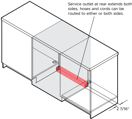
ISO VIEW
