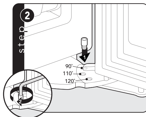
Remove shoulder screw and place in 90° or 120° position.
