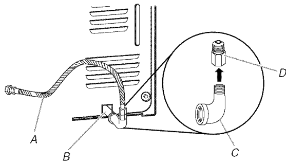
A. 3/8" flexible gas connector B. 3/8" dryer pipe C. 3/8" to 1/2" pipe elbow D. 3/8" pipe-to-flare adapter fitting
