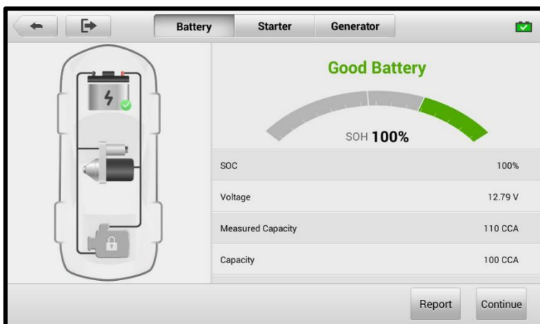
Figure 10-7 Battery Test Results Screen
