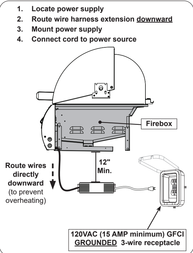
Fig. 30-3 Electrical installation
