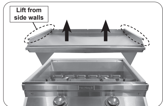
Fig. 28-2 Remove griddle top
