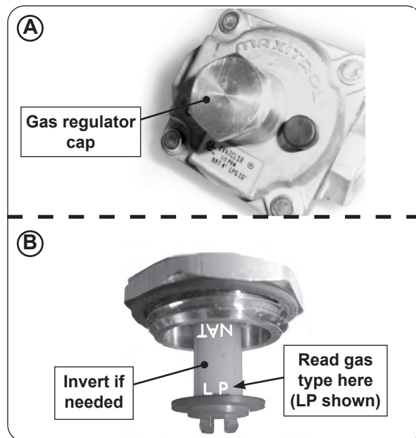
Fig. 43-1 Regulator conversion
