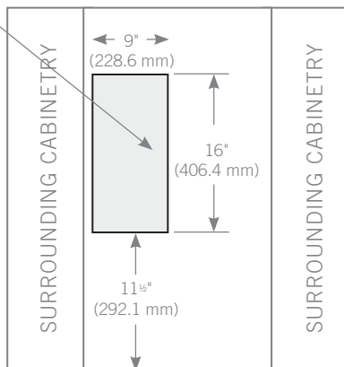
FRONT VIEW OF CABINERY OPENING
