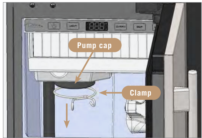
FIG. 1. Pump cap and clamp locations.
