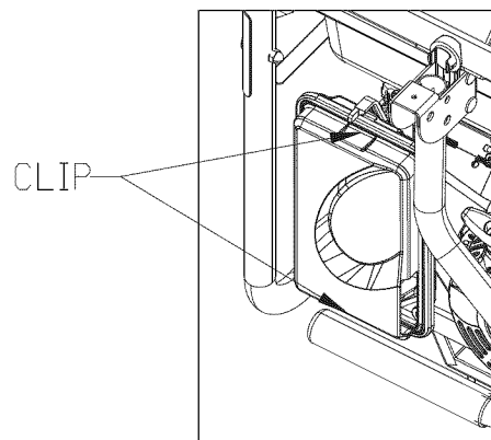
Figure 16 - Air Filter
