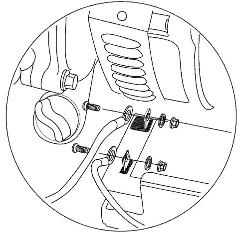
Figure 15 - Battery Connections
