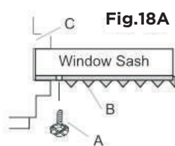
A. 3/4'' (or 1/2'' ) long hex head screw B. Left-hand Window Filler Panel Top Leg C. Window channel
