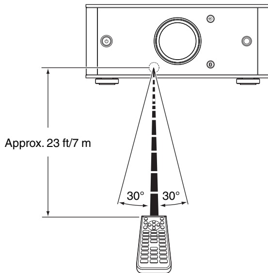
[Horizontal installation]
