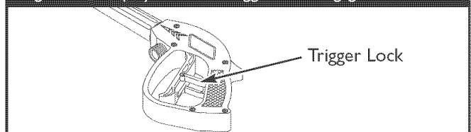
Figure 11 — Spray Gun with Trigger Lock Engaged
