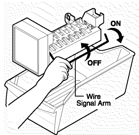
Ice Maker
