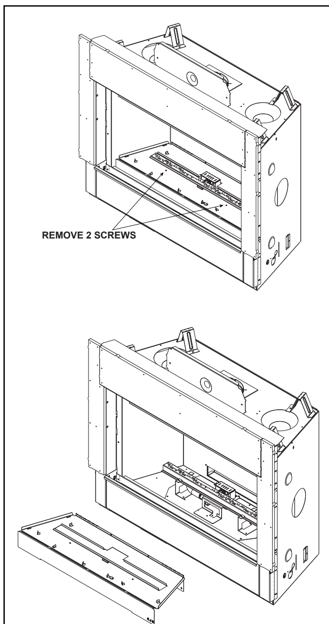
Figure 9.1 Basepan Removal - JADE42IN-B Shown
