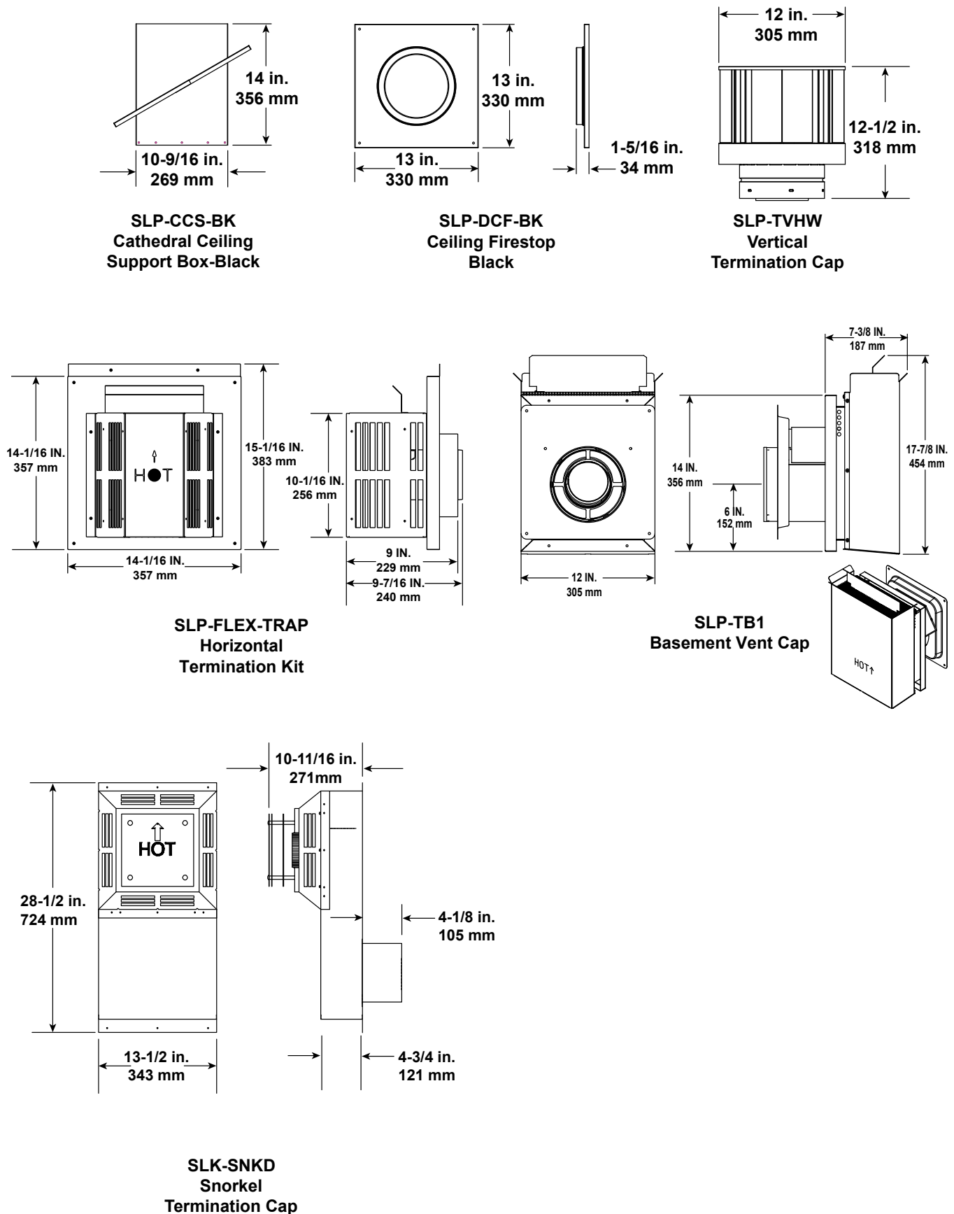
Figure 12.3 SLP Series Vent Components
