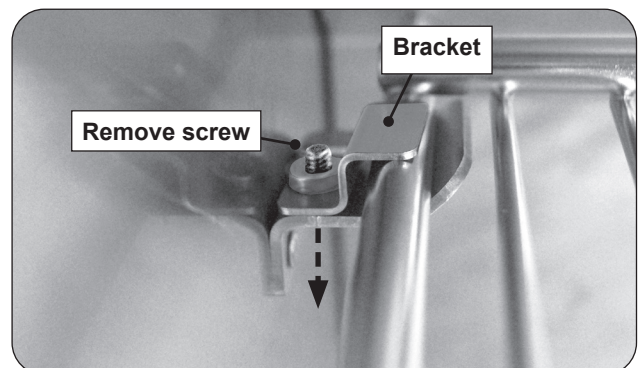
Fig. 38-3 Warming rack locking bracket removal
