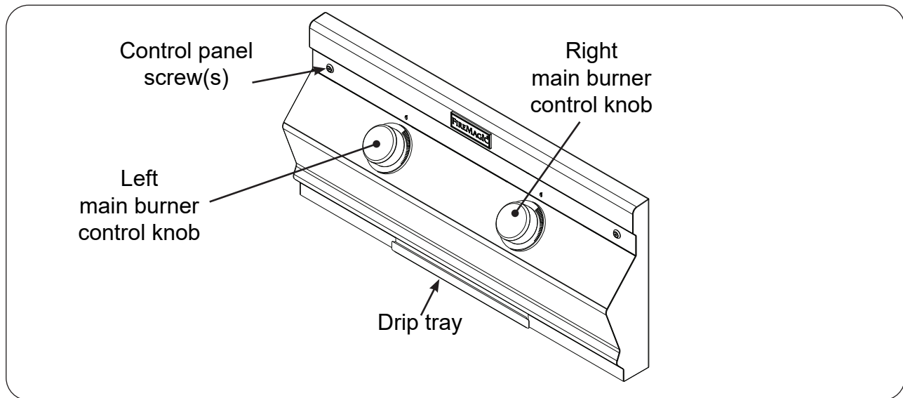
Fig. 30-1 CM430i controls
