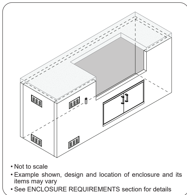
Fig. 25-1 Enclosure construction overview (if applicable)
