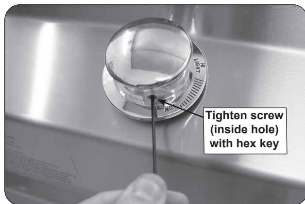
Fig. 29-2 Tighten screw to lock knobs
