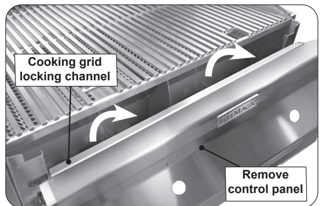
Fig. 36-4 Control panel removal
