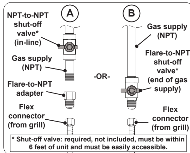
Fig. 27-1 Connecting to a gas line
