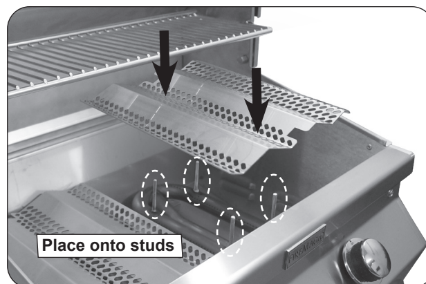
Fig. 27-2 Install flavor grids
