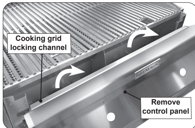
Fig. 37-1 Control panel / grid locking channel removal
