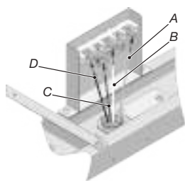
(type A orizontal) 4-WIRE CONNECTION
