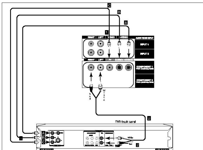
Figure 9. Connecting a DVD Player with Component Video
