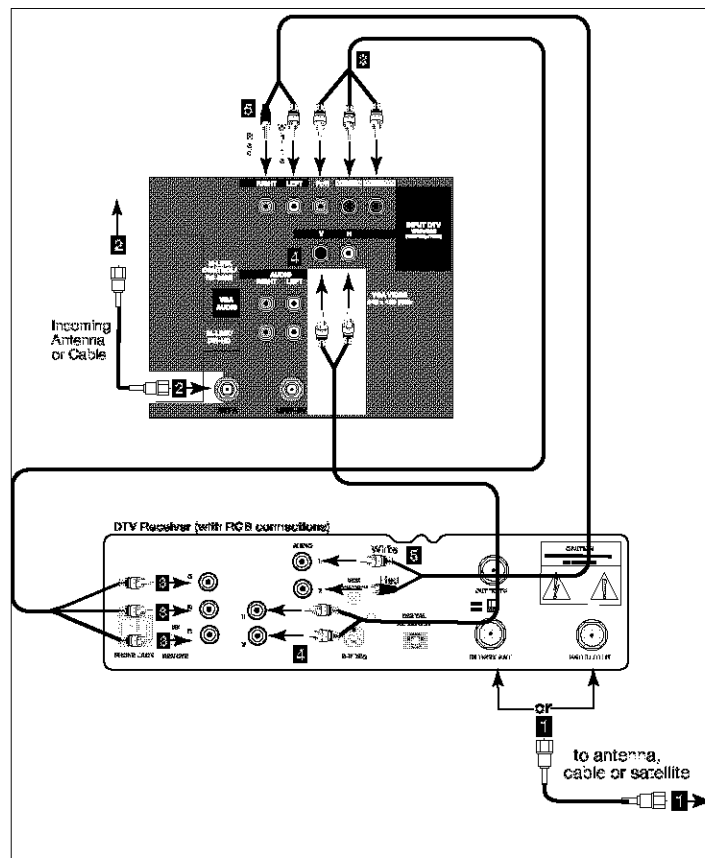
Figure 13. Connecting an External DTV Receiver with RGB, HV Video Connections
