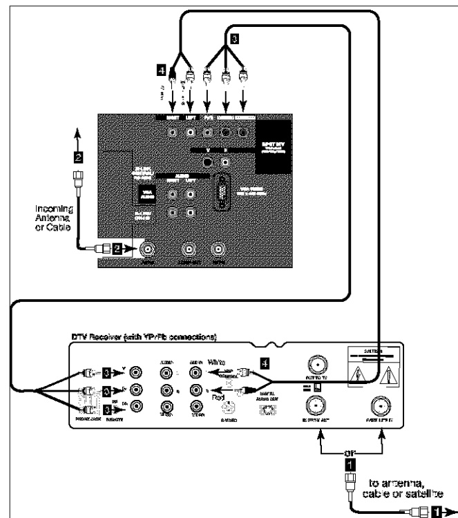
Figure 12. Connecting an External DTV Receiver with Component Video Connections
