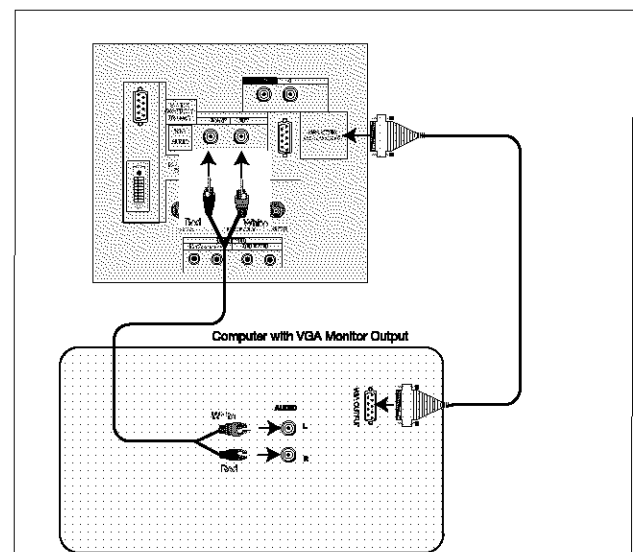
Figure 15. Connecting a Computer with a VGA Monitor
