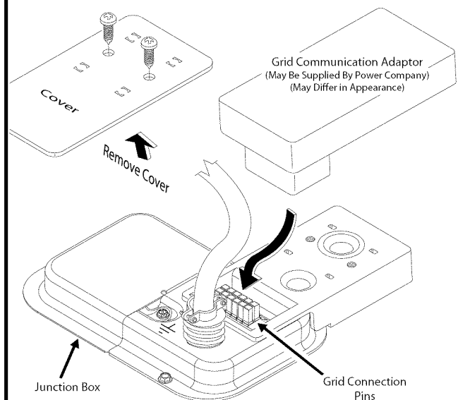
Figure 10C Smart Grid Connection
