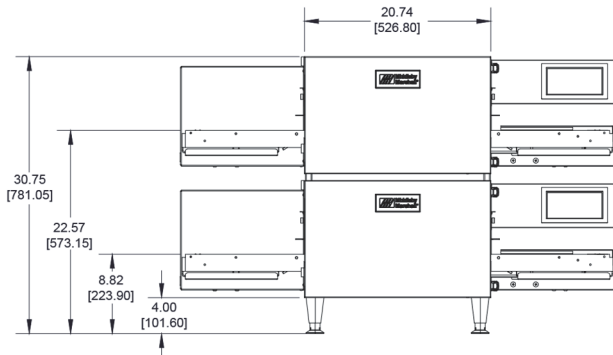
Figure 4: PS2020G Oven Dimensions – Front (Double)
