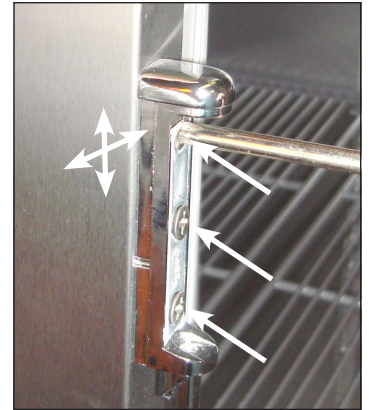
Fig. 4. Door hinge screw locations. Move the hinge as needed.
