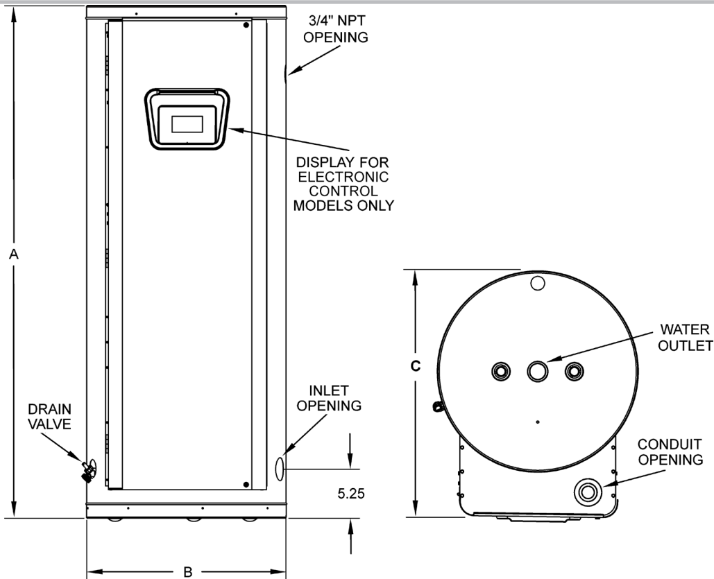
Figure 3. Rough-In Dimensions
