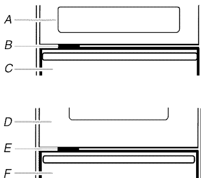
Single Oven Double Oven A. Control panel D. Upper oven B. Oven vent E. Oven vent C. Oven F. Lower oven
