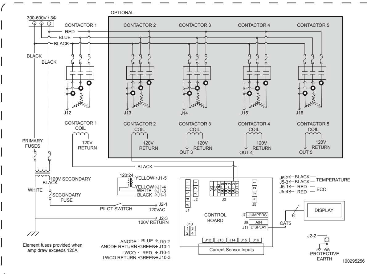
Figure 8. Three Phase Wire Diagram
