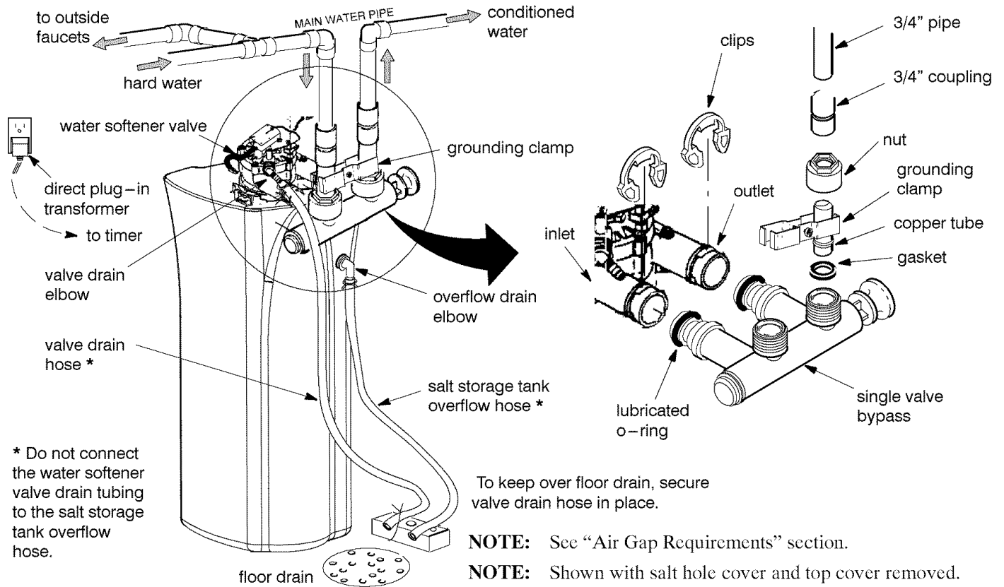
Figure 5 (typical installation)
