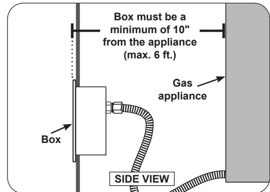
Fig. 2-2 Box clearance
