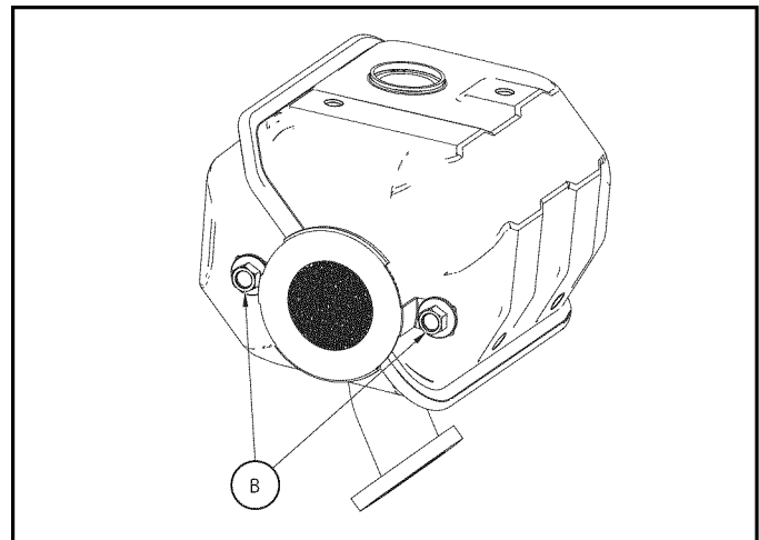
Figure 6-11. Remove Spark Arrester
