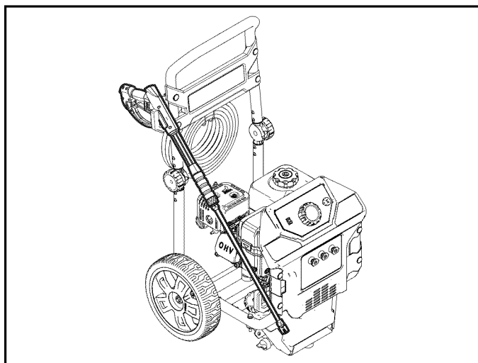
Figure 4-6. Pistolet/lance
