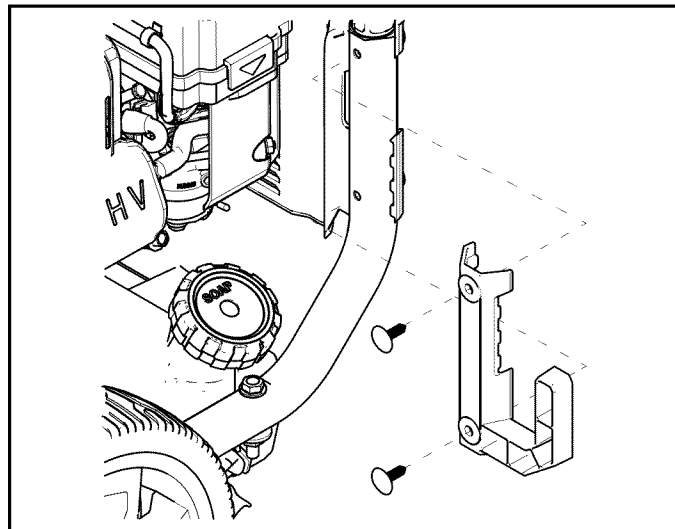
Figure 4-2. Attach Lance Hook to Unit
