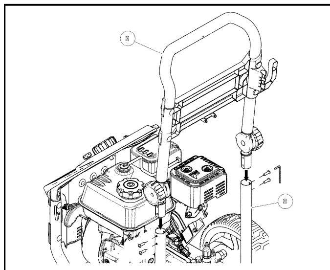
Figure 4-3. Attach Handle to Unit
